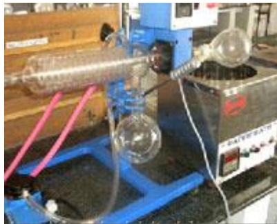
Rotary Vacuum Evaporator
